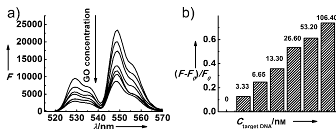
Figure 5. a) Fluorescence emission spectra of the UCP–SA–B–ssDNA complex in the presence of different concentrations of GO (0, 0.02, 0.05, 0.08, 0.10, 0.15, 0.2 mg mL -1 ). b) Restoration of UCP fluorescence after incubation with target ssDNA (0, 3.33, 6.65, 13.3, 26.6, 53.2, 106.4 nM) in the presence of 0.2 mg mL -1 GO.
